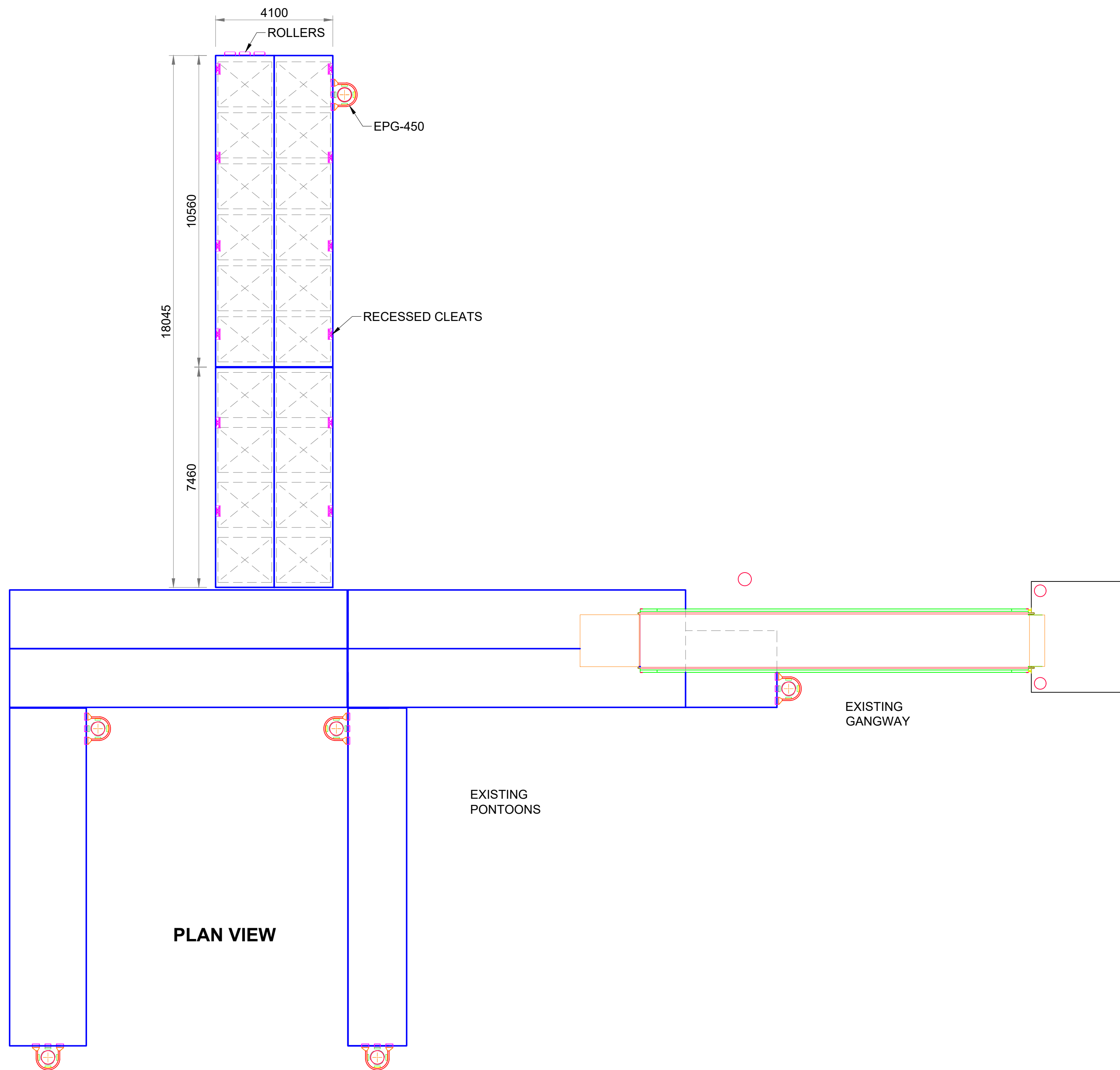
PONTOON LAYOUT SCALE 1 : 100
